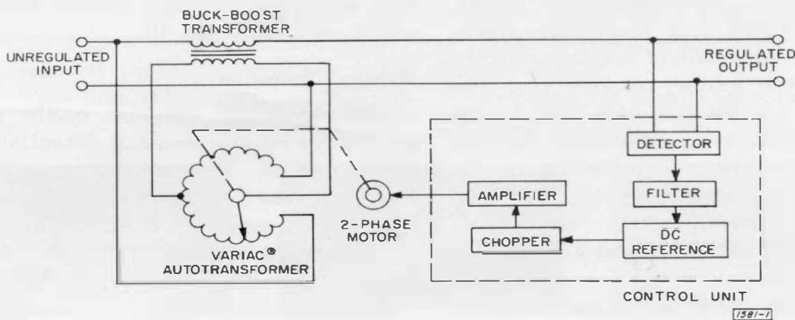
Figure 2. An elementary diagram of General Radio's electromechanical regulator.
