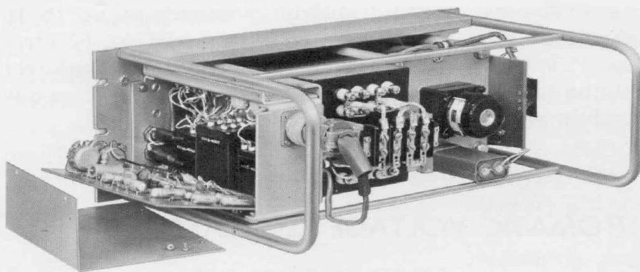
Figure 3. Rear view of a regulator with dust cover removed and etched board swung out for access to components and wiring.
