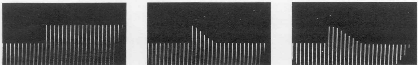
Figure 4. Oscillograms showing response of two of the new regulators to a 2% step change in line voltage. Left, the unregulated input; center, the response of a 6-kVA model; right, the response of a 10-kVA model.
